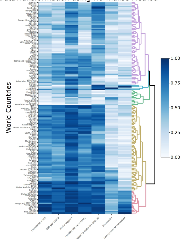
World Happiness Score and Variables by Country, 2018 DataTransformation using Normalise Method
