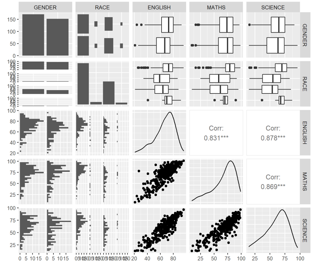
Generalised Pairs Plot
